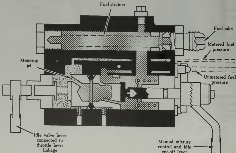
FIGURE 3-33. Fuel metering section of the injector.
